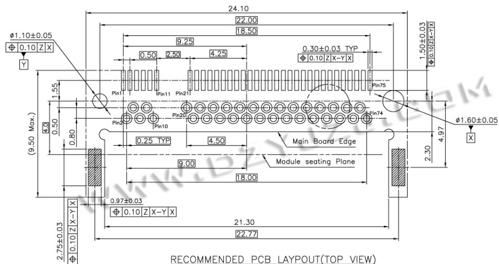
RECOMMENDED PCB LAYOUT(TOP VIEW) DEFAULT TOLERANCE±0.05
